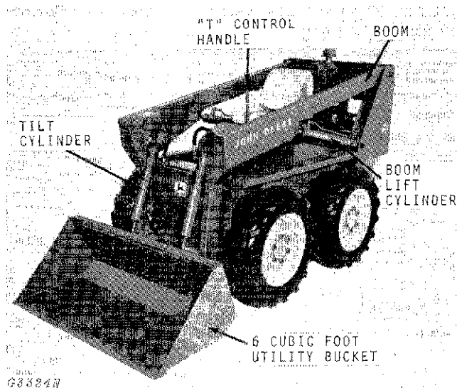
Fig. 1-70 Skid-Steer Loader
