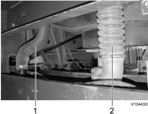
Figure 19 Disconnect, radiator and charge air cooler hose
