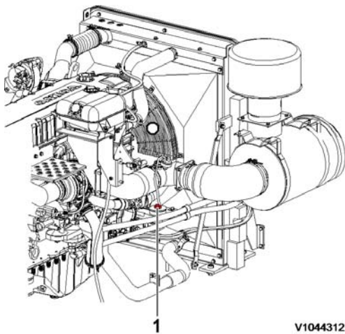
Figure 1 Installation, engine
